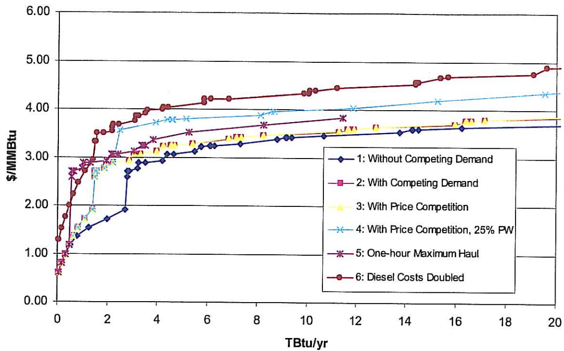
Figure 13. Results of the six scenarios for the GRU Deerhaven facility.
