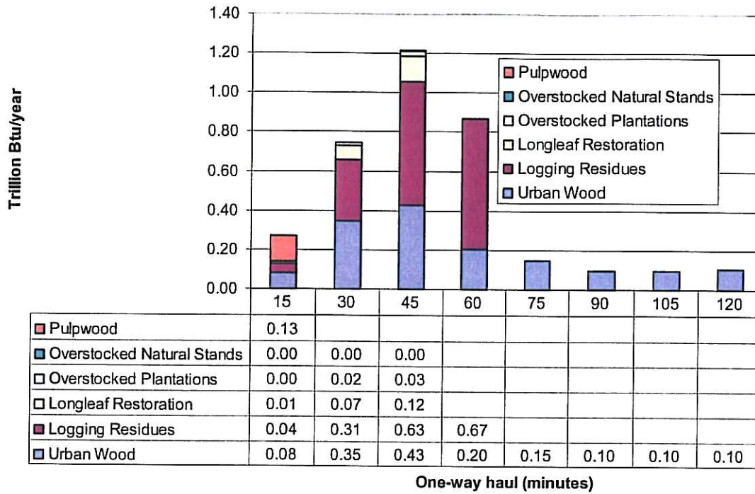
Figure 14. Biomass use profile up to 3.55 TBtu/year (40 MW) for the JEA Brandy Branch facility under scenario #2, "With competing demand".
