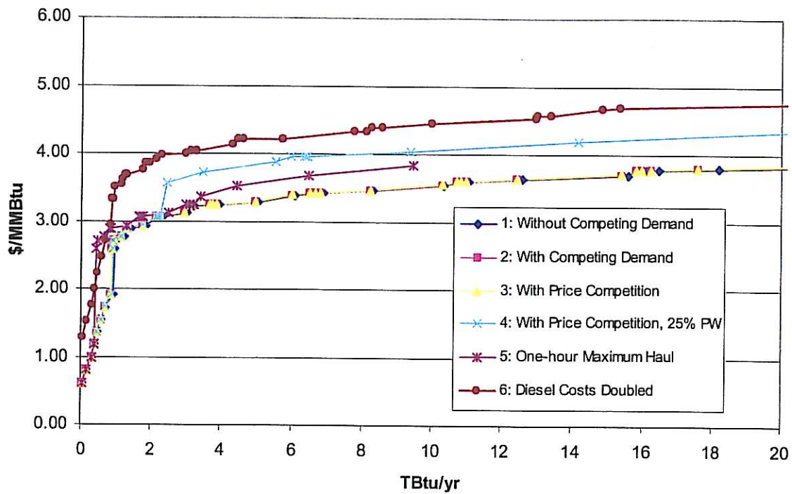
Figure 17. Results of the six scenarios for the TAL Hopkins facility.
