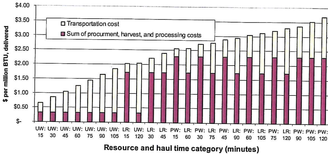
Figure 5. Transportation costs and sum of procurement, harvest, and processing costs of urban wood waste (UW), logging residues (LR), and pulpwood (PW) within a two-hour haul travel time at fifteen minute intervals. Transportation costs include loading and unloading costs.
