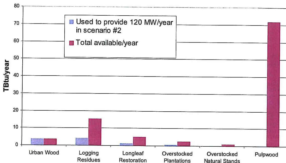
Figure 33. A comparison of A) least-cost resources used to provide 10.65 TBtu/year (three 40 MW facilities) under scenarios #2: “With competing demand” and #3: “With price competition”, and B) total availability of these resources within the three two-hour woodsheds, excluding overlap of adjacent woodsheds.
