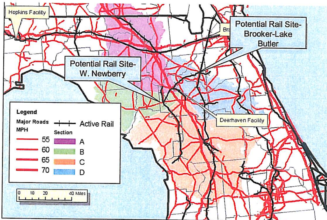
Figure 29. Potential rail concentration yard sites.
